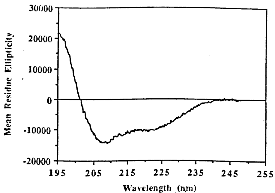
FIG. 5. Far ultraviolet CD spectra of insulin extracted from 1-octanol using an aqueous solution of 0.10 M HCl. The pathlength was 1 mm, the sample concentration was 53 \mu\text{g/ml} , and the sample temperature was 5° C.
